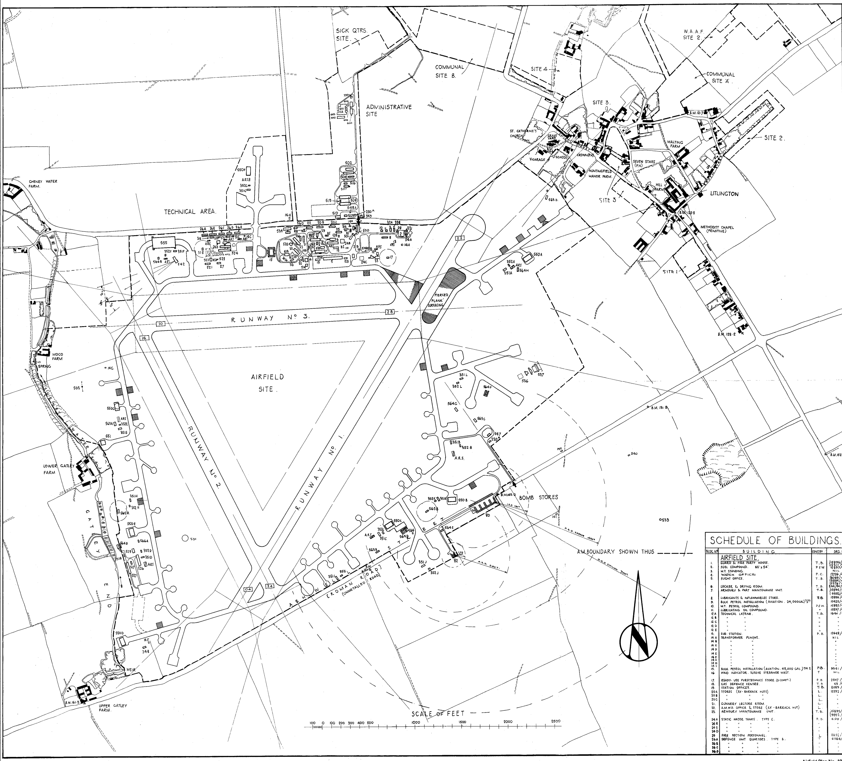
BASED ON O.S. SHEETS C.A.M.S. LVIII. NE & SE. LOCATION PLAN STEPPLE MORDEN
